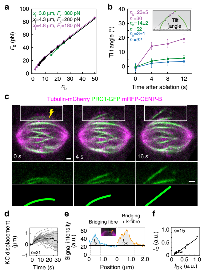
Figure 4 | Force at the spindle pole increases with the number of MTs in the bridging fibre. (a) Force at the pole, F_0 , as a function of the number of MTs in the central part of the bridging fibre, n_b . The inputs of the model are
